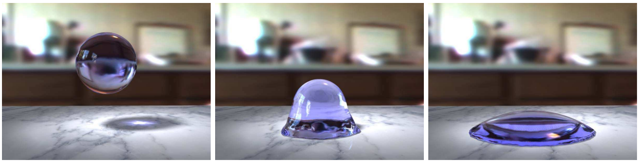
Fig. 7: A droplet falling onto a hydrophilic surface.
